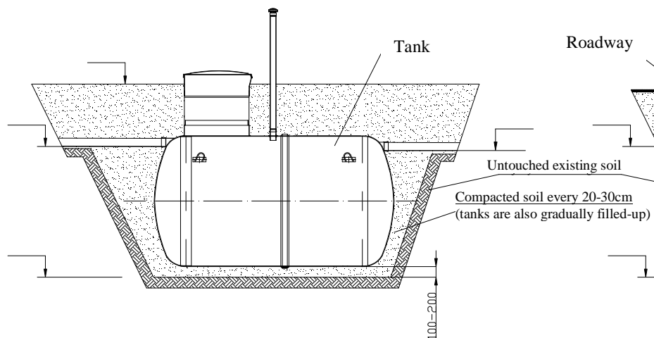
ANCHORAGE OF HORIZONTAL TANK
