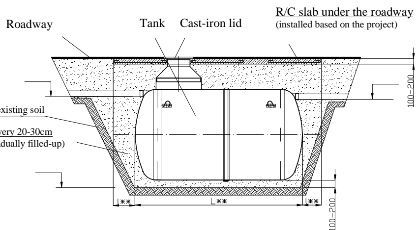
INSTALLATION OF HORIZONTAL TANK ON THE ROADWAY
