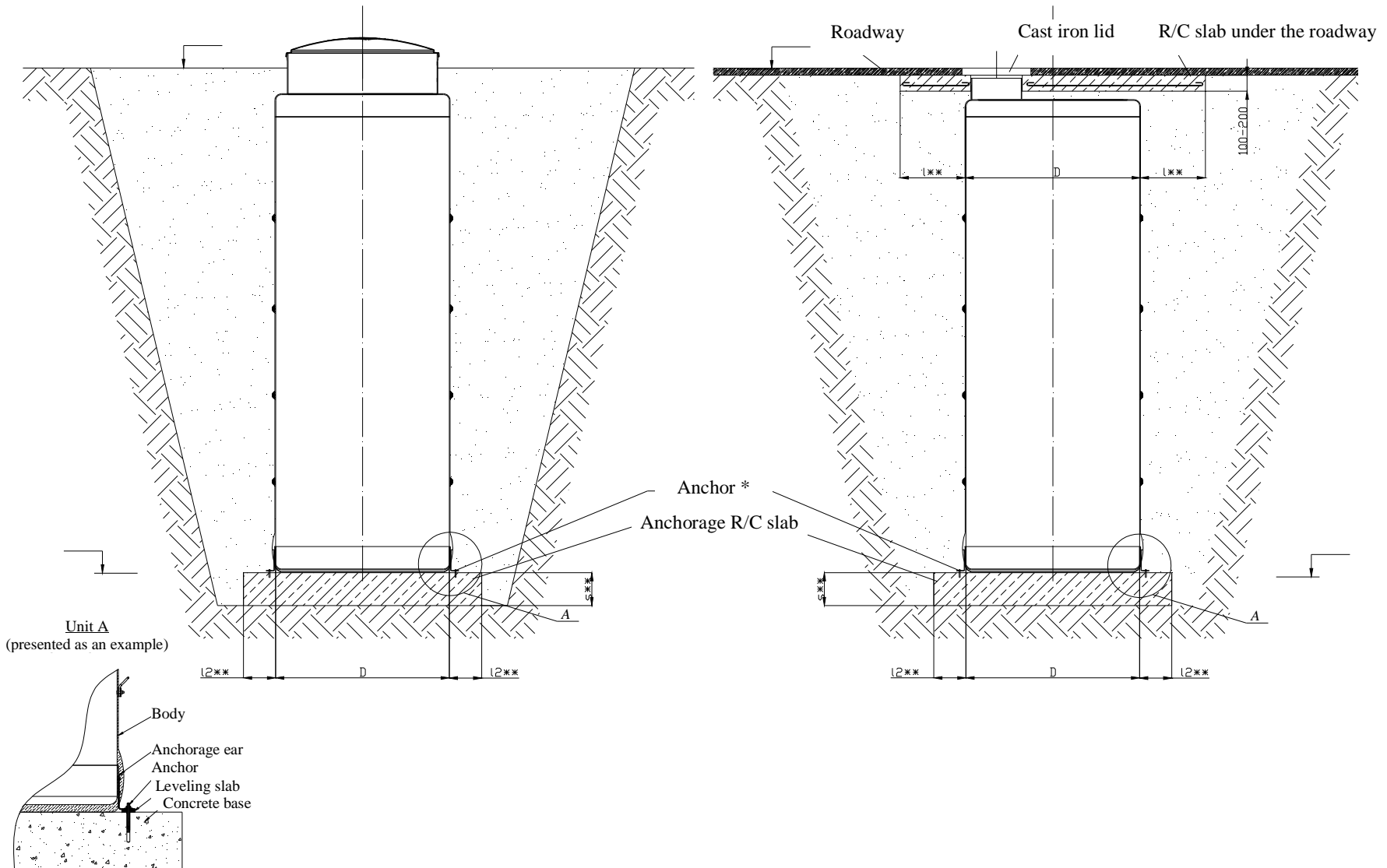
INSTALLATION OF VERTICAL TANK IN GREEN LAWN
