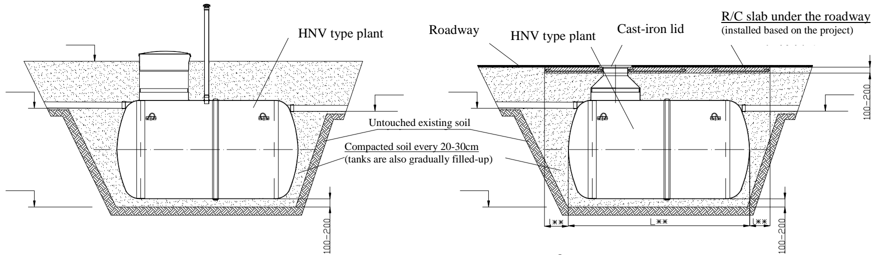
ANCHORAGE OF HNV type TREATMENT PLANT
